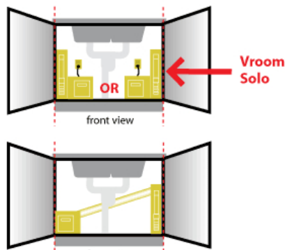
VROOM SOLO for standalone use (Vacuum unit incl.)
